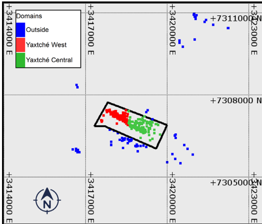
Figure 14-2: Yaxtché Domains with All Drill Hole Collars in the Database
