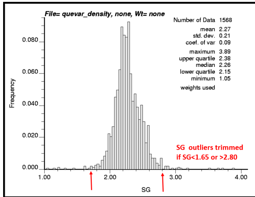
Figure 14-16: Histogram of SG Values Showing Lower and Upper Trimming
