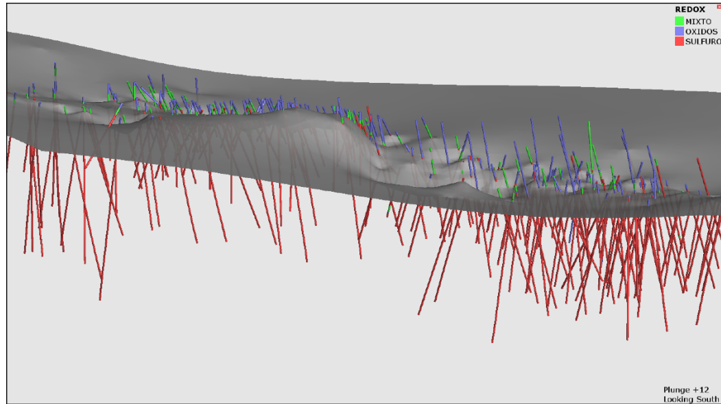
Figure 14-13: Perspective View Looking South of the Oxide-Mixed-Sulfide Codes and the DTM used to Delineate Oxide and Sulfide in the Resource Model
