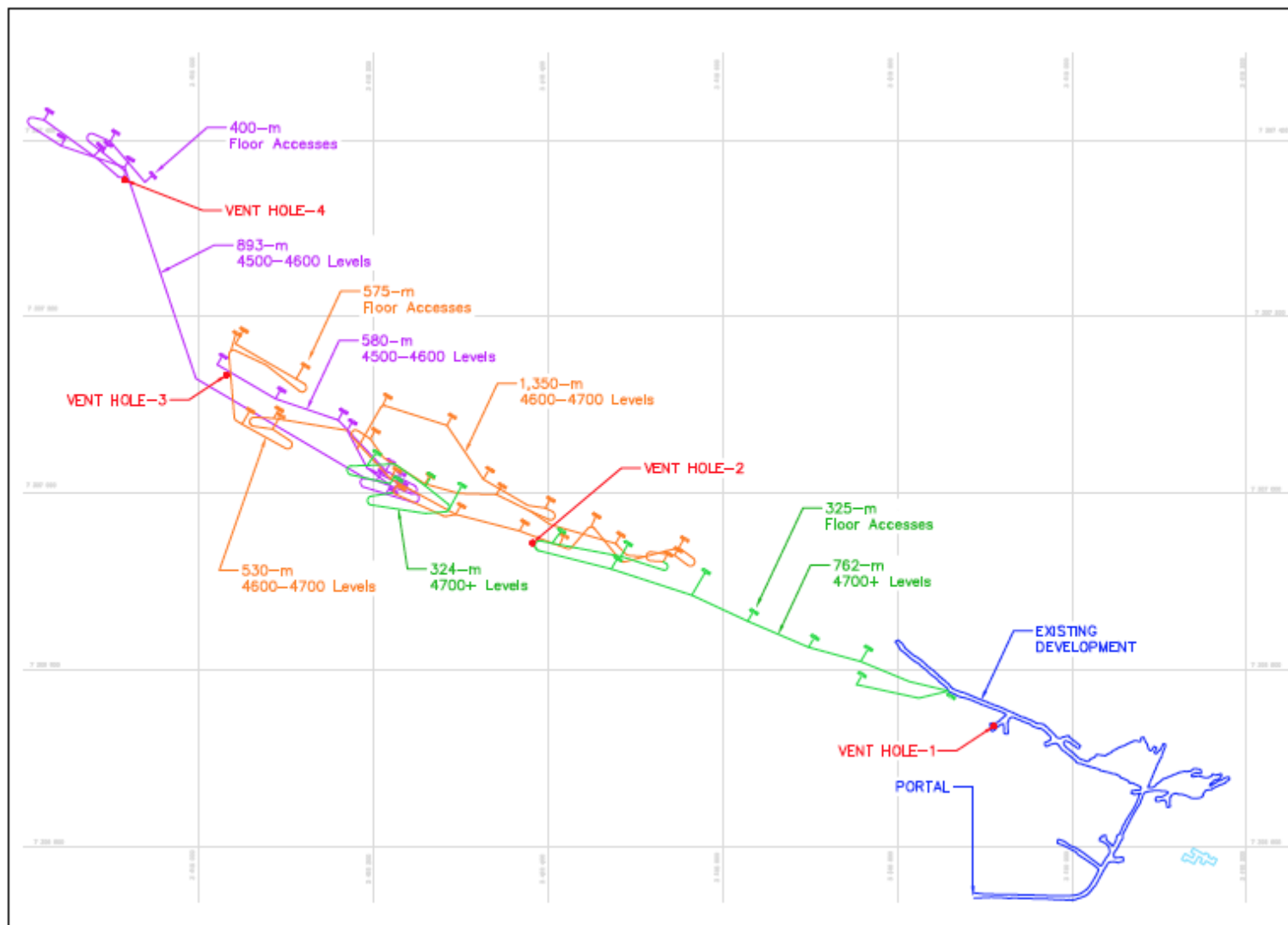
Figure 16-2: Planned Mine Development
