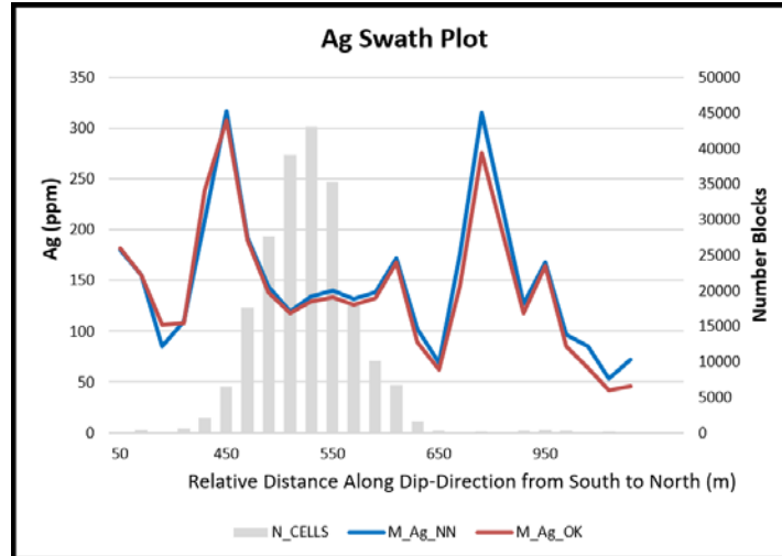
Figure 14-21: Ag Grade Trends Along Dip-Direction
