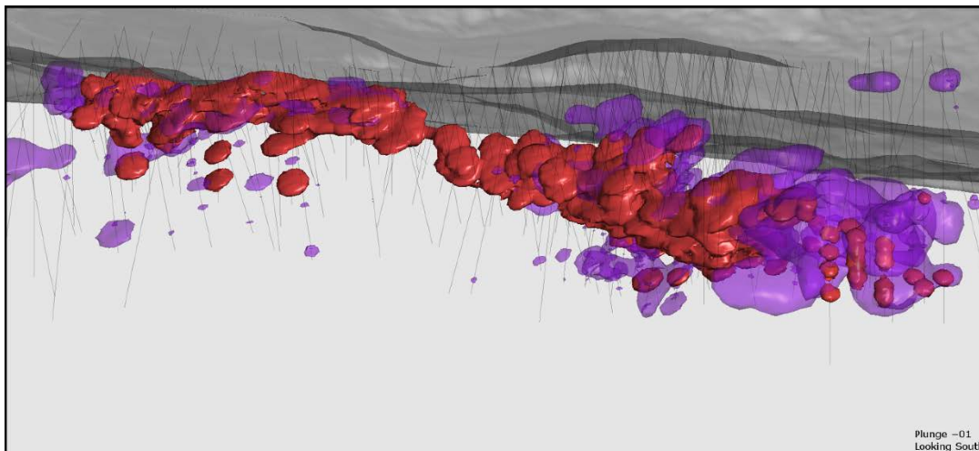
Figure 14-6: Perspective View Looking South of the 150 g/t Ag Shell (Red) in Relation to Pb Mineralization (Purple)
