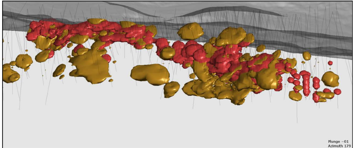
Figure 14-8: Perspective View Looking South of the 150 g/t Ag Shell (Red) in Relation to the As Mineralization (Brown)
