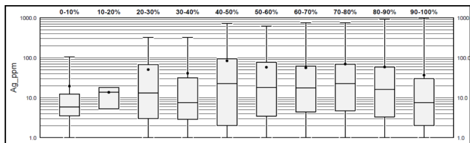
Figure 14-4: Yaxtché Central, Ag Grades Categorized by Core Recovery
