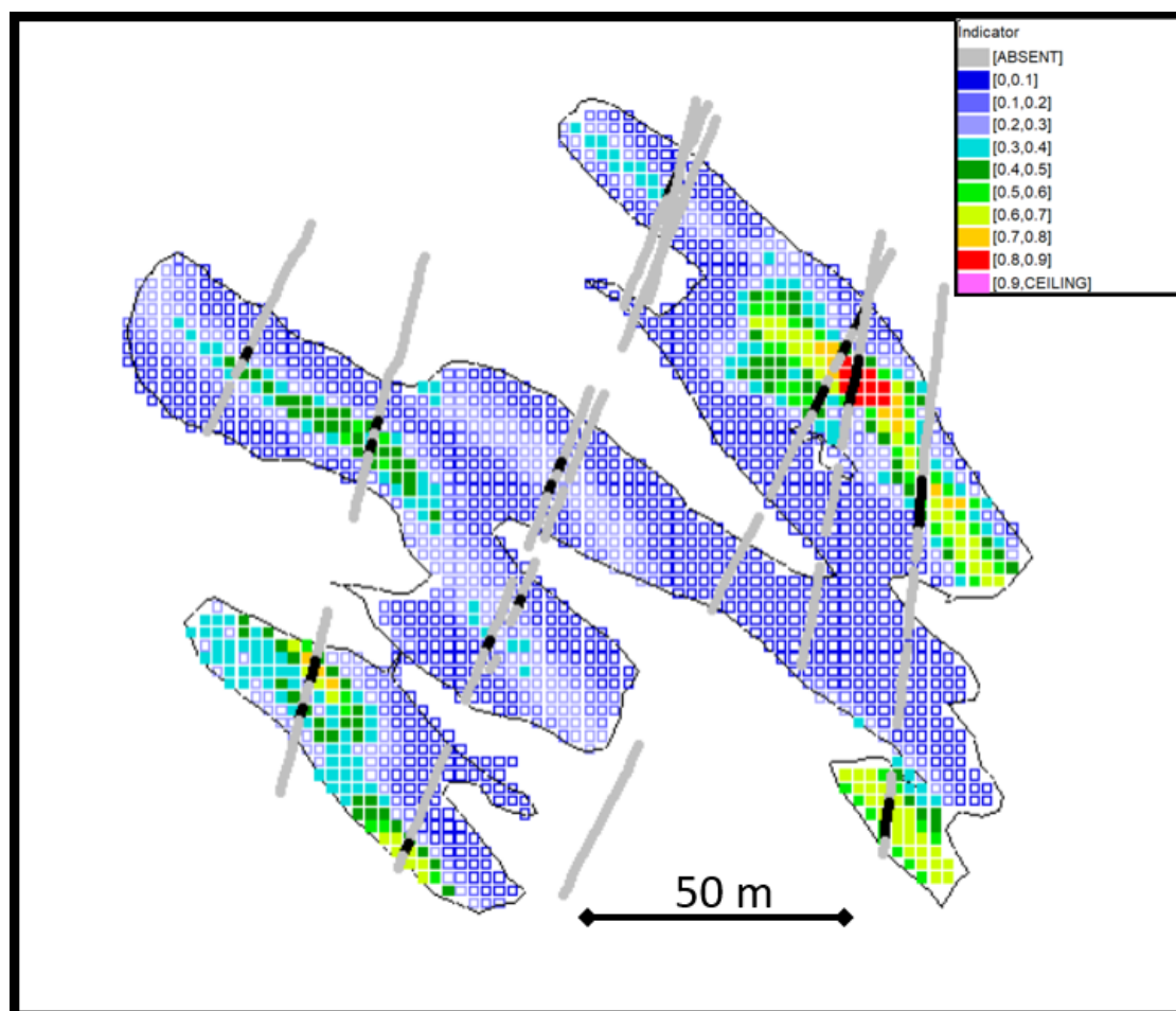
Figure 14-18: Example of Indicator Model
