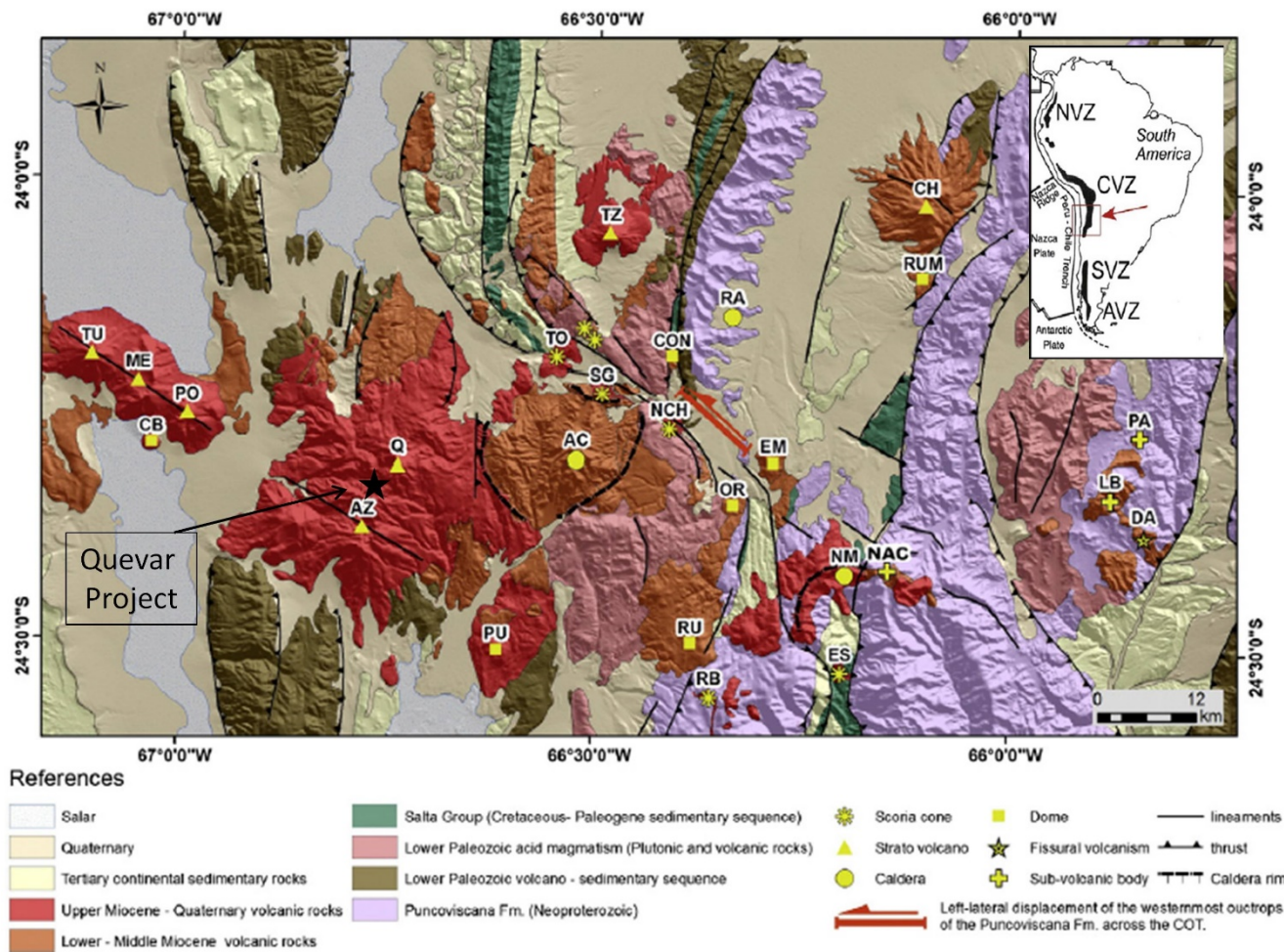
Figure 7-1: Regional Geology Plan
