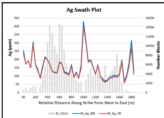
Figure 14-20: Ag Grade Trends Along Strike
