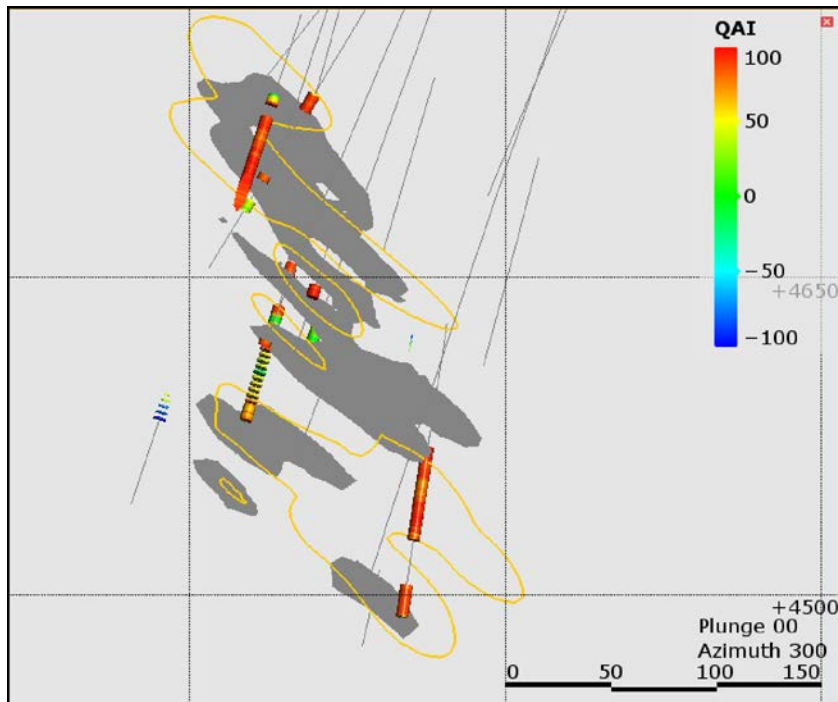
Figure 14-11: Cross Section Looking 300° Showing the 150 g/t Ag Shell (Dark Gray) in Relation to the Alteration Index (QAI) (Yellow)
