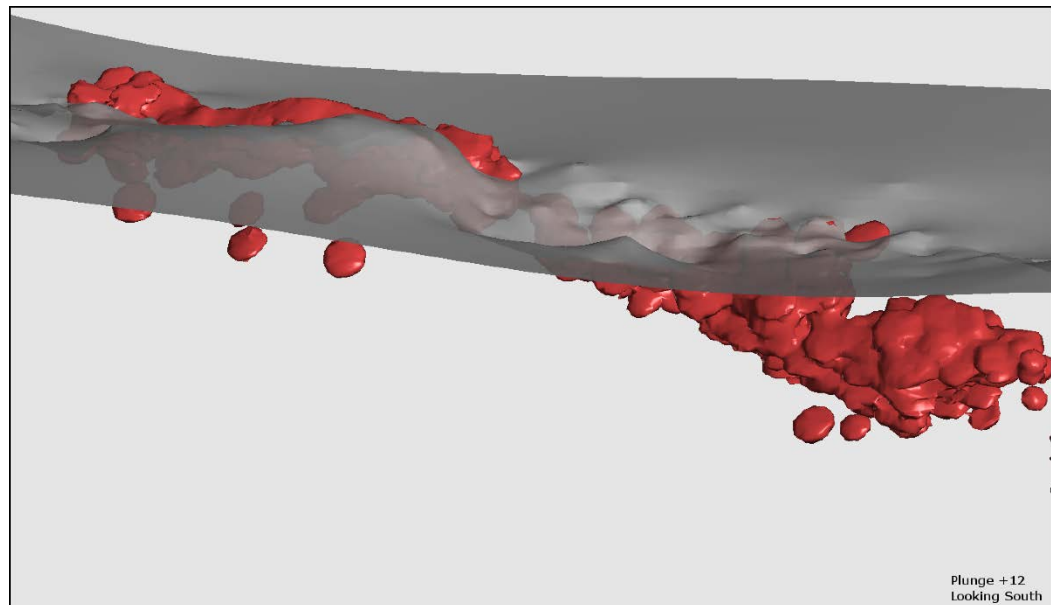
Figure 14-14: Perspective View Looking South 150 g/t Ag Shell and the DTM used to Delineate Oxide and Sulfide in the Resource Model
