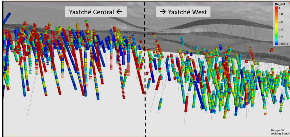
Figure 14-1: Example of Element Zonation Between Yaxtché West and Central Using Na%
