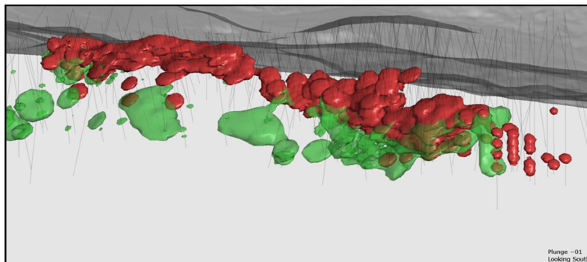
Figure 14-5: Perspective View Looking South of the 150 g/t Ag Shell (red) in Relation to Cu Mineralization (green)
