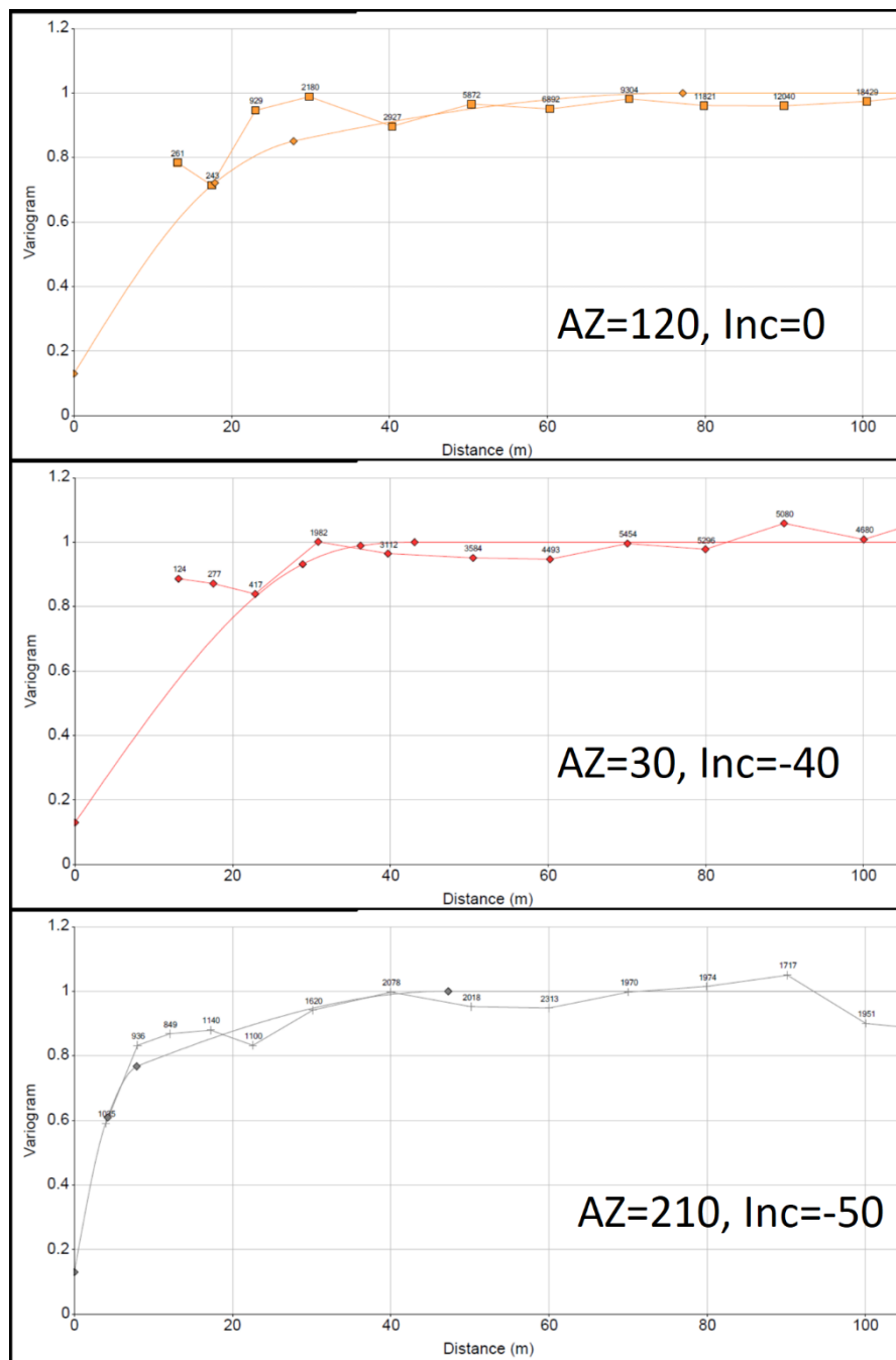
Figure 14-17: Example Variograms for Ag
