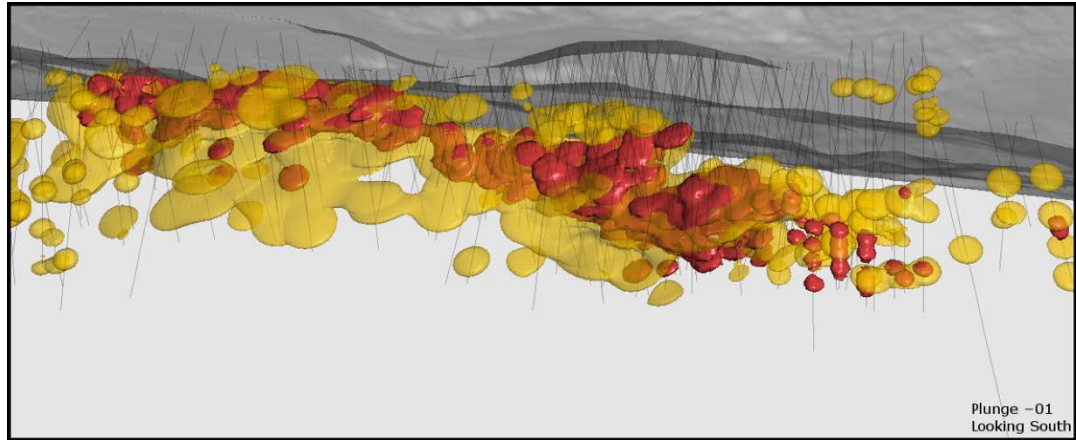
Figure 14-10: Perspective View Looking South of the 150 g/t Ag Shell (Red) in Relation to the Quevar Alteration Index (QAI) (Yellow)
