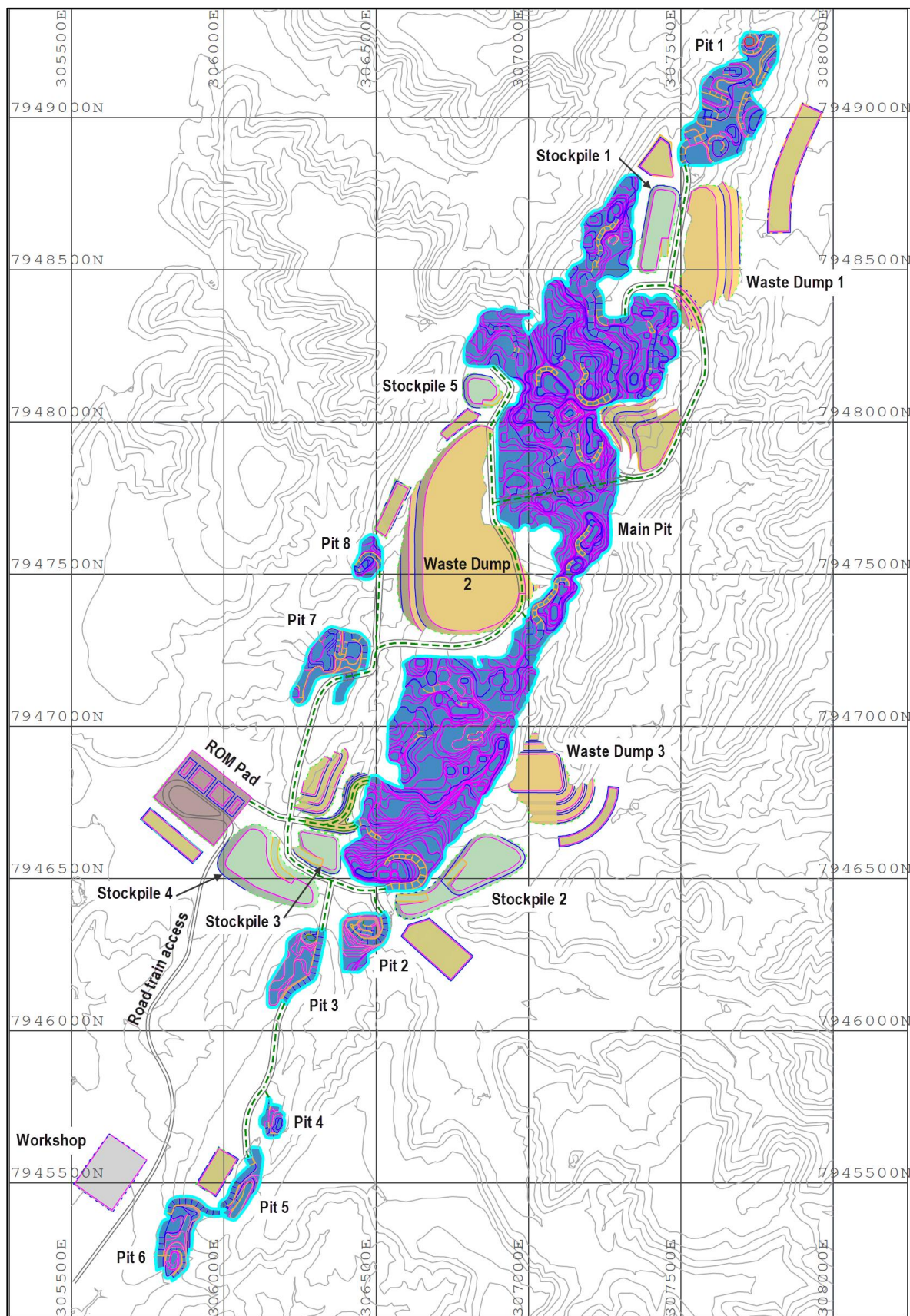
Figure 4: Proposed site layout of the Kokomo mining operation
