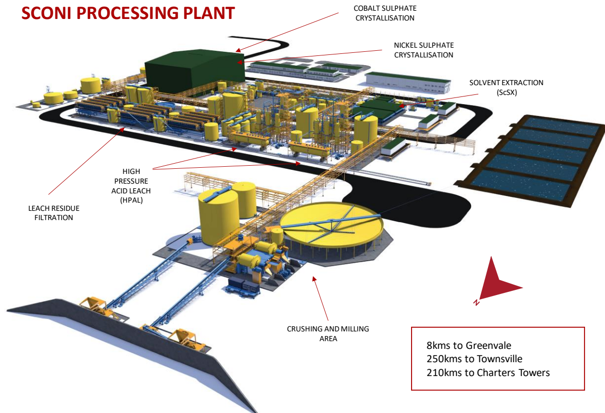
Figure 8: Indicative design for the Sconi Project's processing plant located close to the historic mining town of Greenvale
