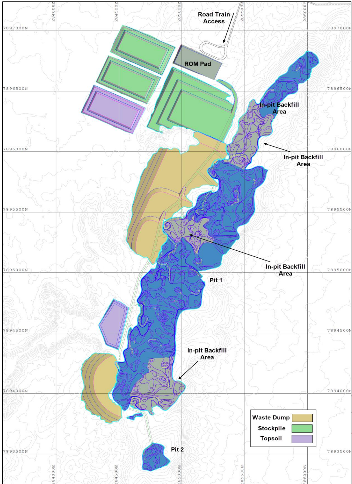
Figure 3: Proposed site layout of the Lucknow mining operation
